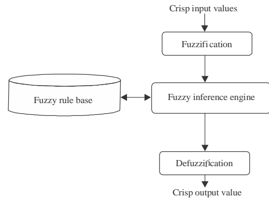
Fig. 1: Fuzzy logic mode
