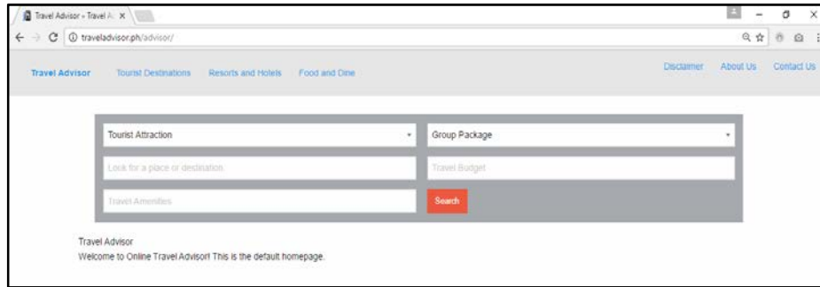
Fig. 4: Search function
