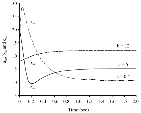
Fig. 5: Time history of the parameter estimates (Theorem 1)
