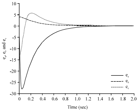
Fig. 6: Time history of the parameter estimation errors (Theorem 1)
