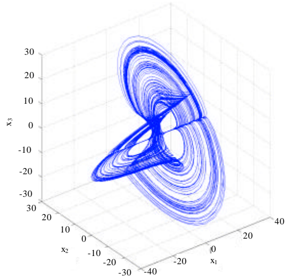
Fig. 1: The 4-scroll attractor of the Liu-Chen system
