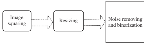
Fig. 3: Pre-processing steps
