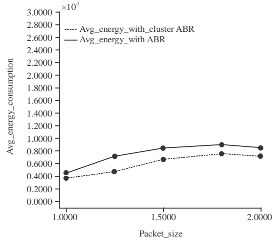
Fig. 7: Packet size vs. average energy consumption
