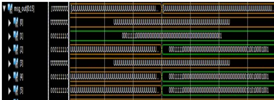
Fig. 8: BQ packet with the source and destination address and the sequence number attached at node 1. Node 1’s neighbours (2, 4 and 5) receiving the packet
