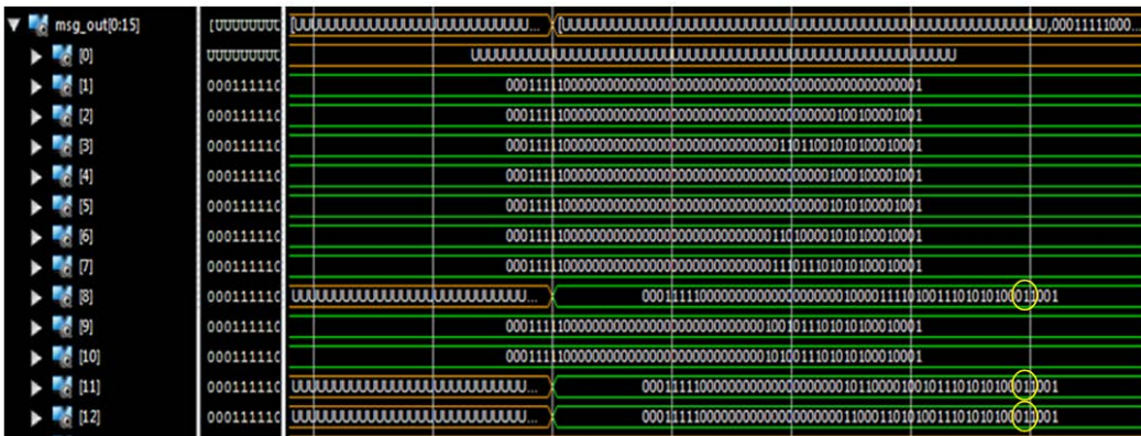
Fig. 11: Nodes 8, 11 and 12 receive the BQ packet and increment hop count to 3 (Yellow circle: Bits 5 down to 3)
