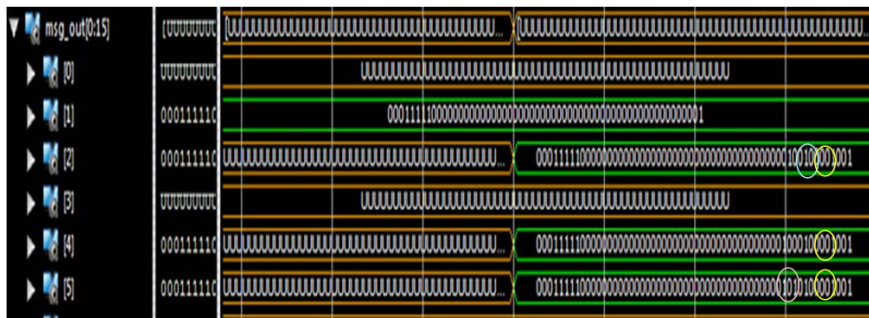
Fig. 9: Neighbours 2, 4 and 5 attach their respective addresses (White circle: Bits 13 down to 10) and associativity ticks (Light Blue circle: Bits 9 down to 6) and increment the hop count to 1 (Yellow circle: Bits 5 down to 3)
