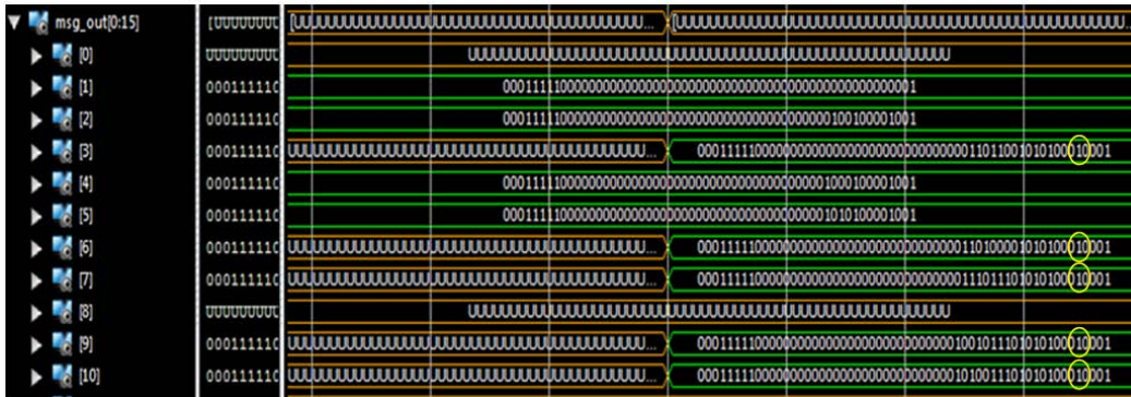
Fig. 10: Nodes 3, 6, 7, 9 and 10 receive BQ packets from various nodes and increment the hop count to 2 (Yellow circle: Bits 5 down to 3)
