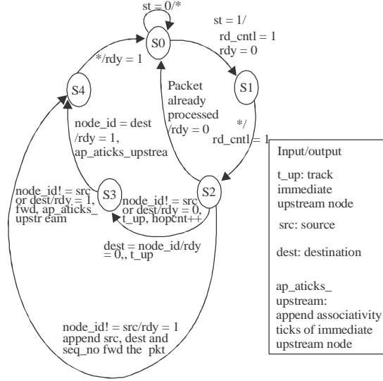
Fig. 4: State diagram of a node during route construction (Broadcast query packet transmission)
