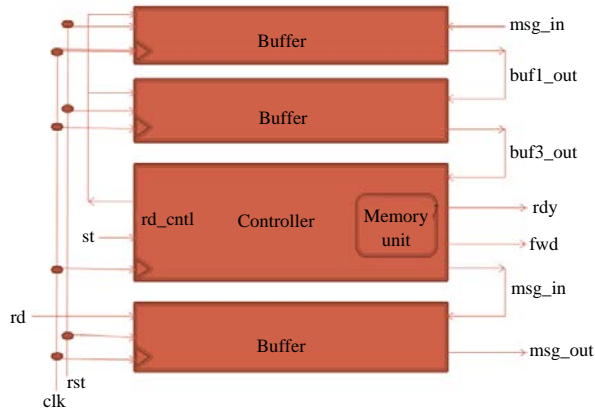
Fig. 3: Implementation of a node
