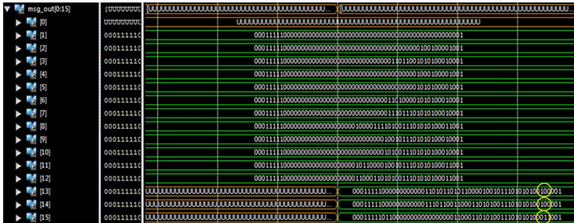
Fig. 12: Nodes 13, 14 receive the BQ packet and increment hop count to 4 (Yellow circle: Bits 5 down to 3). Destination node 15 receives the first BQ packet
