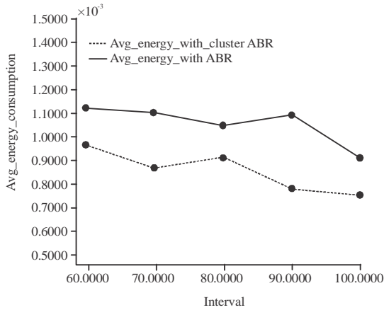
Fig. 6: Interval vs. average energy consumption
