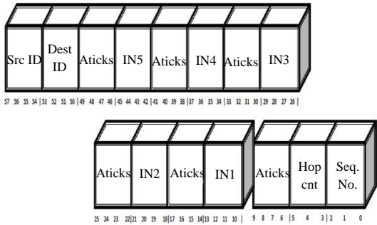
Fig. 2: Broadcast query packet format
