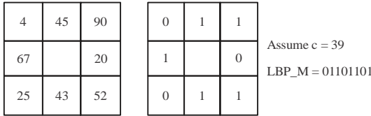
Fig. 5: LBP_M operator
