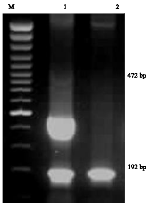
Fig. 2: Duplex PCR method for detection of differentiation of capripoxvirus. M-100 bp ladder; Two amplicons of 472 and 191 bp are obtained in case GPV samples representing fusion and attachment gene fragments respectively, while only 191 bp attachment gene fragments got amplified from SPV samples
