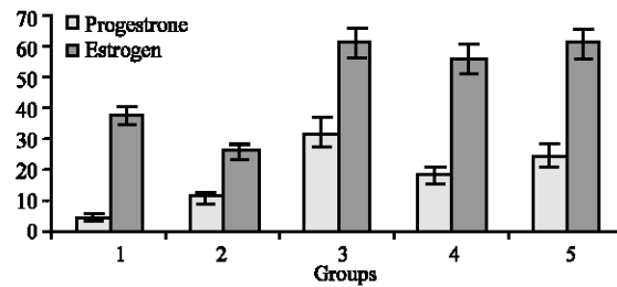
Fig. 3: Effect of gonadotrophin on ovarian estrogen and progesterone synthesis
