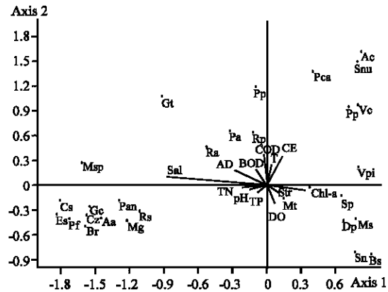
Fig. 3: CCA (Canonical correspondence analysis) of water parameters withcay Creek
