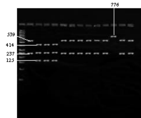
Fig. 3: Electrofresing digested product on agarose gel: marker 50 bp
