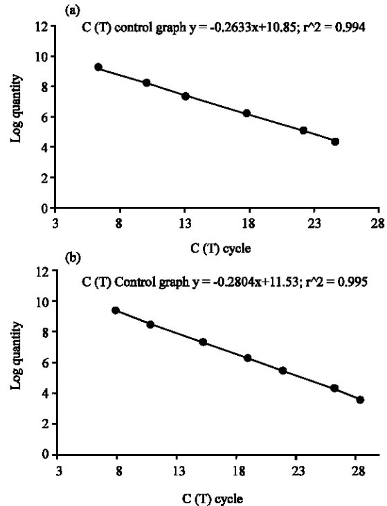
Fig. 1: Standard curve obtained by plotting the logarithm of the DNA concentration for anaerobic fungi (a) and methanogenic archaea (b) versus threshold cycle (C (T)) mean values
