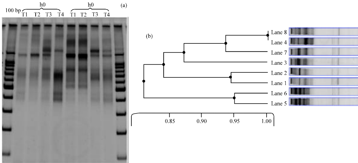
Fig. 2: Negative image of SYBR ® Gold stained denaturing gradient gel electrophoresis separation pattern of eight PCR samples in which the rumen anaerobic fungi ITS1 amplicon from rumen content of buffalo (T1 = RS, T2 = RS+4% urea, T3 = ULRS+0% urea and T4 = ULRS+4% urea) are shown (a) along with the corresponding cluster analysis of the sample profiles (b)
