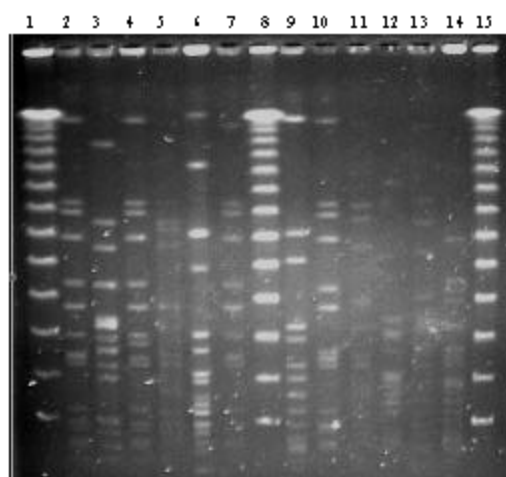
Fig 1: Presentation of the profiles of PFGE of the strains of Staphylococcus aureus after digestion by the SmaI endonuclease. Lanes; 1, 8 and 15: Scorer of size of molecular weight. 48, 5-1000 kb (λ-ladder Bio-Rad). Lane 9: Strains of reference ((No ATCC: 29213). Lanes 2, 3, 4, 5, 6, 7, 10, 11, 12, 13 and 14: Strains of Staphylococcus aureus
