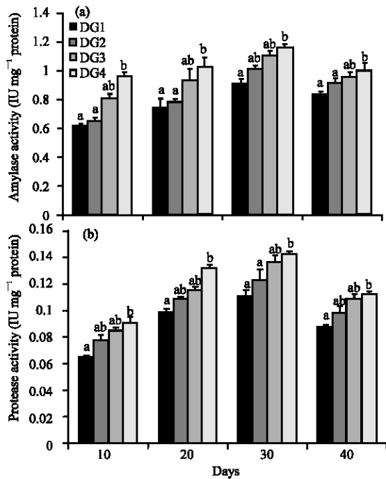
Fig. 1: Specific activity of enzymes in digestive gland of C. catla fed with different experimental diets. Statistical differences ( p < 0.05 ) among groups are indicated by different letters. No significant differences appear among the groups marked with the same letter. DG1-DG4 are represented diet group I-IV, respectively
