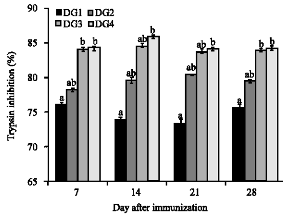
Fig. 2: Fish were immunized with rabbit RBC. Control groups were fed with normal diet and the experimental groups were fed with experimental diet. Total 4 weeks prior to immunization till the end of the experiment. Serum was collected from individual fishes for 4 weeks after immunization. The percentage of trypsin inhibition for each individual serum was determined. The values represented were the mean \pm SE of 4 fishes ( p < 0.05 ). DG1-DG4 are represented diet group I-IV, respectively
