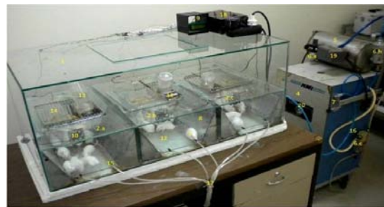
Fig. 1: Appearance of DE Model; 1: DEC (Dry Eye Cabinet); 2 (a-c): EAD (Experimental Animal Division); 3: The subjects; 4: AC (Air compressor); 5: AC tube; 6 (a-c): Water separator; 7: Flowmeter; 8: Desiccators' containers, 9: Control board; 10: Fan; 11: Humidity-Temperature monitor; 12: Mobile glass plates; 13: Watering; 14: Feeder; 15: Air inlet holes; 16: Pneumatic pipes; 17: Flexible inhalation hose; 18: Fan switch board; 19: AC pressure monitor; 20: AC pressure gauge
