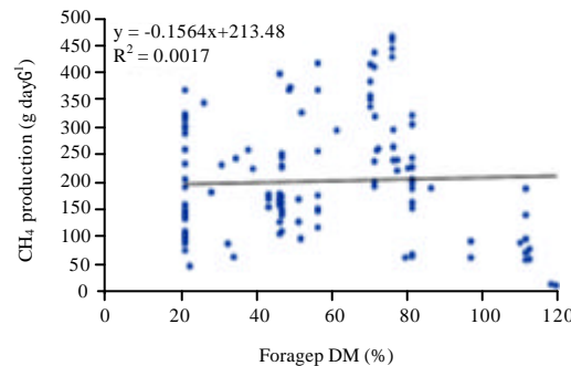
Fig. 5: Relationship of CH 4 production (g day -1 ) with the amount of forage as a percentage of dietary dry matter (forageDM, %)
