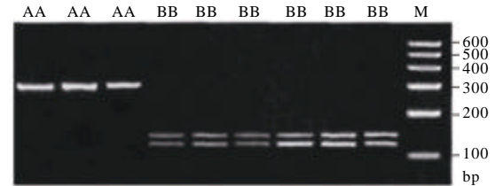
Fig. 2: RFLP agarose gel electrophoresis of COX II gene
