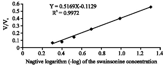
Fig. 3: Calibration curve for swainsonine assay. The calibration curve was obtained by plotting the ratio of inhibited reaction rate to control mannosidase reaction rate ( V_i/V_c ) versus negative logarithm (-log) of the swainsonine concentration
