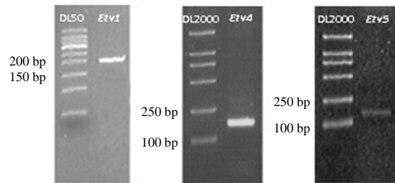
Fig. 1: RT-PCR analysis of Etv1, Etv4 and Etv5
