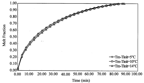
Fig. 5: Comparison of melt fraction of Paraffin Wax with different values of (T_m - T_{ini}) for copper with constant value of T_{wall} - T_m = 15^\circ\text{C}
