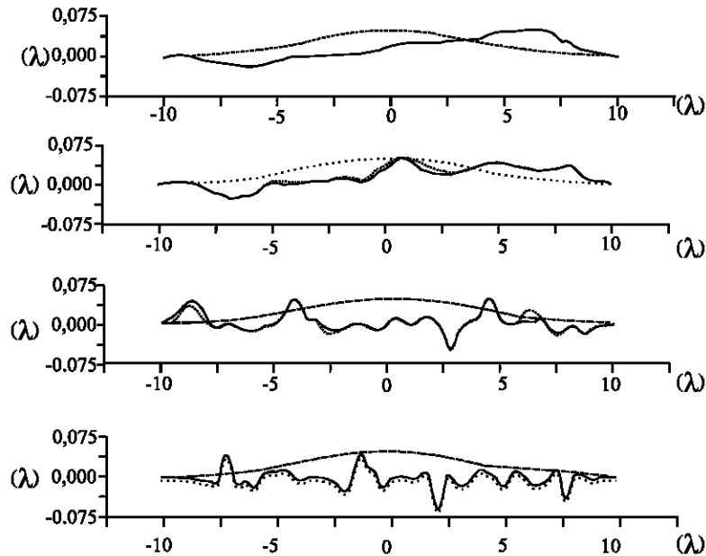
Fig. 4: Reconstruction profile of random surface (a) IT=1 (b) IT=10 (c) IT=30 , (d) IT=100 (—) True profile (---) Estimate, (.....) Reconstruction profile
