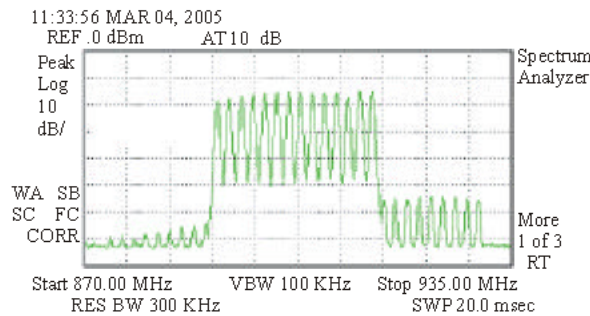
Fig. 6: The ESCP signal as seen at the IFR 3413 output
