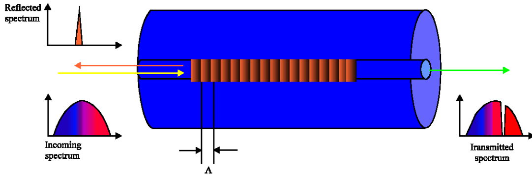
Fig. 1: Schematic description of the fiber Bragg grating
