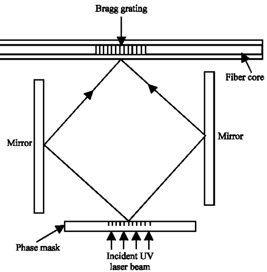
Fig. 9: Schematic diagram of the Talbot interferometer
