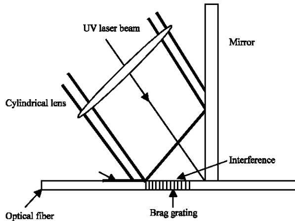
Fig. 5: A schematic of the Lloyd wavefront-splitting interferometer
