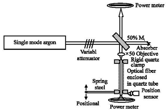
Fig. 2: A typical apparatus used for generating self-induced Bragg gratings
