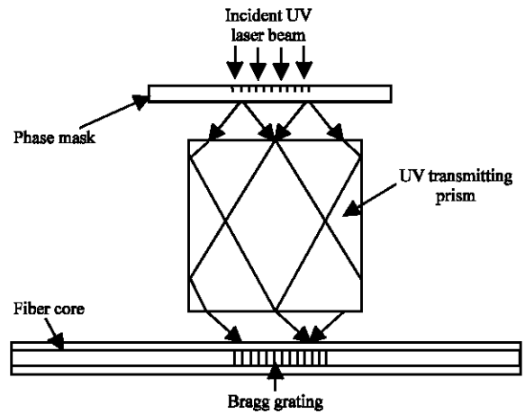
Fig. 8: Noncontact, interferometric phase mask technique
