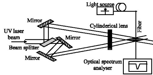
Fig. 3: Amplitude-splitting interferometer
