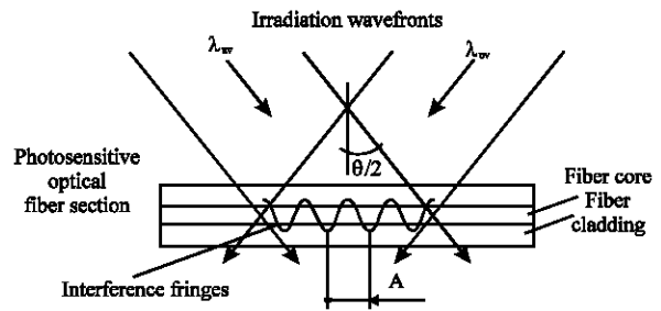
Fig. 4: Interference fringes induced by two interfering UV beam
