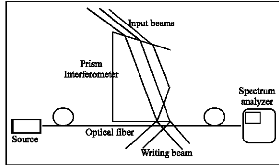
Fig. 6: A schematic of the prism wavefront-splitting interferometer
