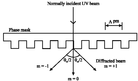
Fig. 12: Schematic of the UV radiation at normal incidence of a phase masks
