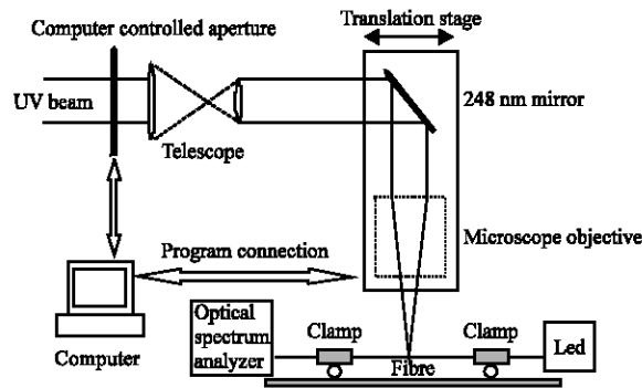
Fig. 11: A schematic setup for writing Bragg gratings using point-by-point technique
