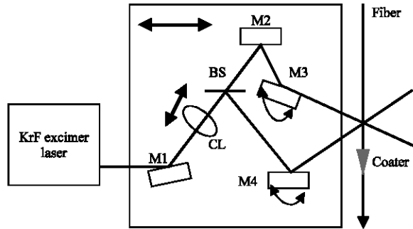
Fig. 10: Schematic of the interferometer to write gratings during fiber draw
