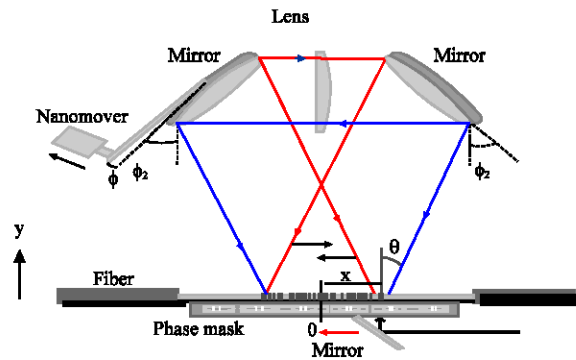
Fig. 7: Sagnac interferometric phase mask technique
