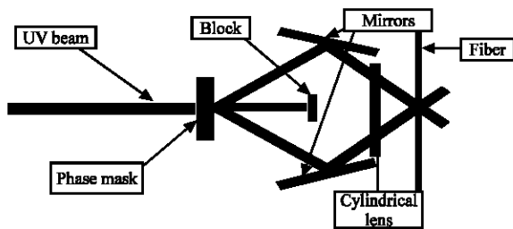
Fig. 15: A schematic setup of a modified phase mask technique
