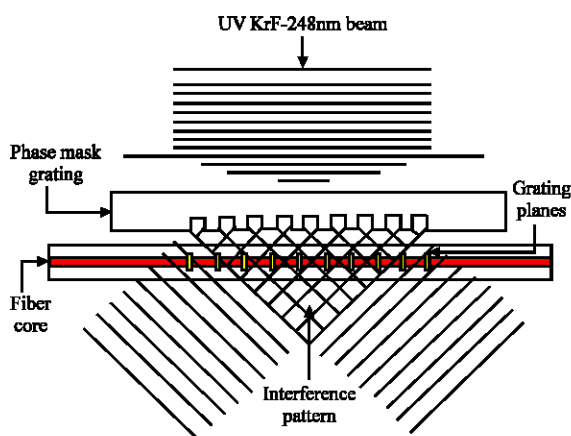
Fig. 13: The interference pattern photoimprints a refractive-index modulation in the core of a photosensitive optical fiber
