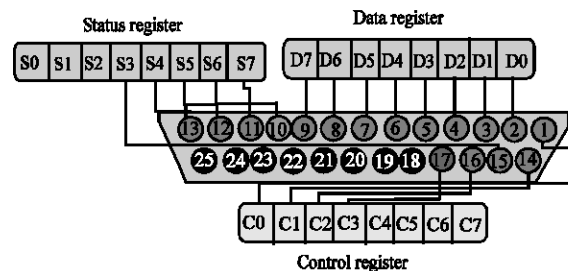
Fig. 1: Parallel port pin status
