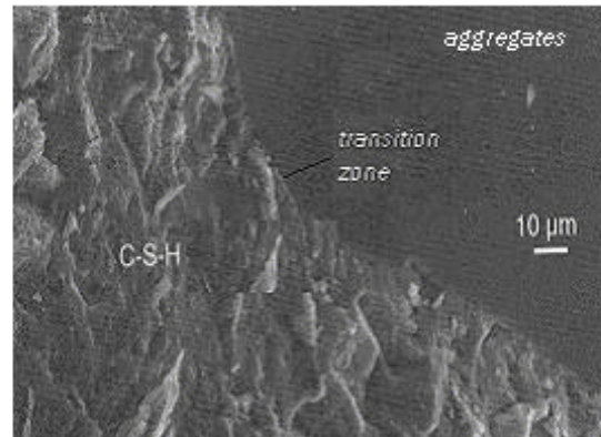
Fig 3: Dense C-S-H around the aggregate in concrete with silica fume
