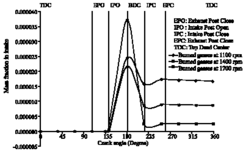
Fig. 9: Effect of mass fraction for burned gases in intake at different engine speed and porting
