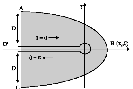
Fig. 1: The configuration of the flow. The x-axis is along the horizontal flat board and the y-axis is vertically through the tip system of the board
