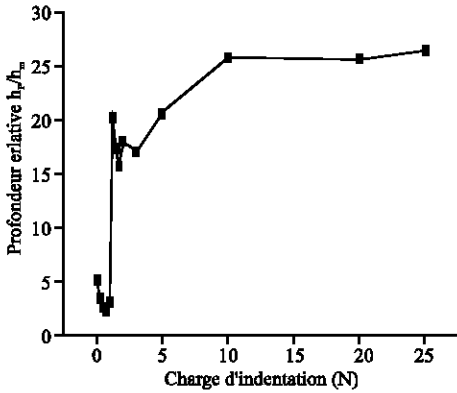
Fig. 4: Evolution of the report h_v/h_m as a function of indentation load
