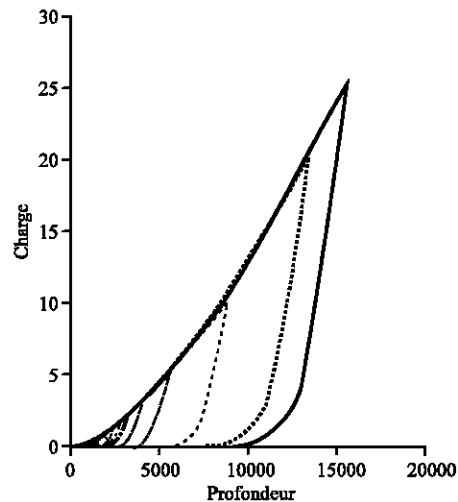
Fig. 3. Load-displacement curve
