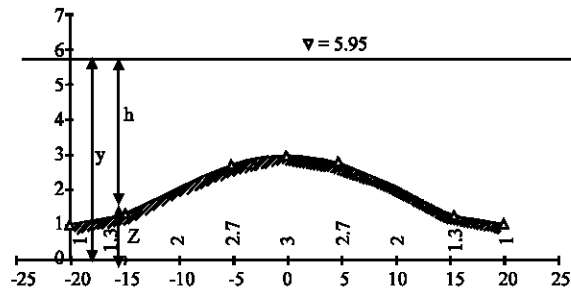
Fig. 8: Diagram of the initial bed situation
