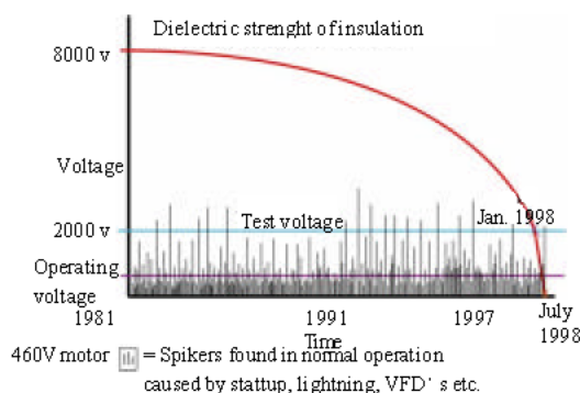
Fig. 7: Dielectric strenght insulation degradation (Curtis, 2002)
