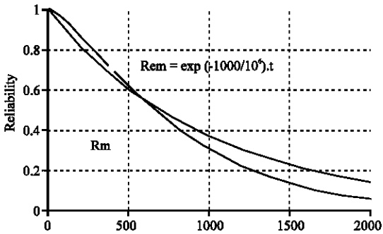
Fig. 12: Graphical comparison of the overall reliability of the induction motor with an exponential form reliability of constant failure rate ( \sim 1 \text{ F}/1000\text{h} )
