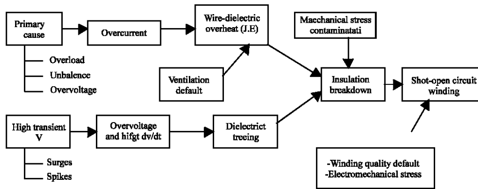
Fig. 2: Failure mechanisms sequence of the electrical stator windings
