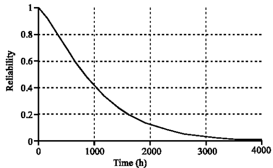
Fig. 10: Reliability evolution of the rotor
