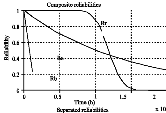
Fig. 11: The overall reliability of the electric AC motor
