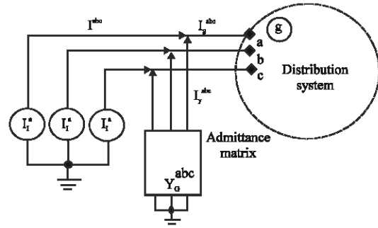
Fig. 11: Norton's equivalent circuit of cogenerator
