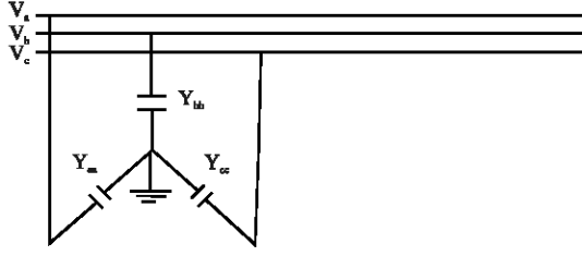
Fig. 6: Capacitors connected in wye connection
