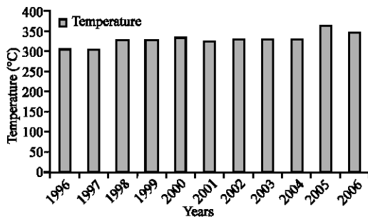
Fig. 4: Annual temperature (1996-2006)
