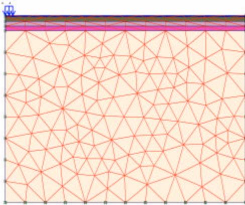
Fig. 3: Finite elements meshes
