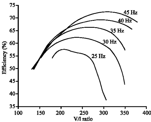
Fig. 5: V/I ratio vs. efficiency at different modulating frequency
