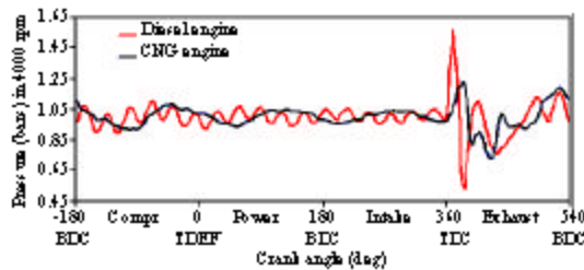
Fig. 10: CNG engine and diesel engine intake port static pressure in 4000 rpm
