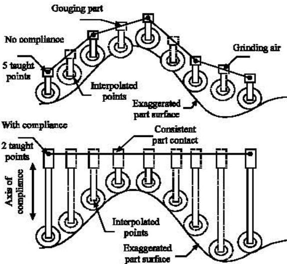
Fig. 8: Illustration of the compliance on surface contact
