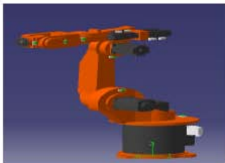
Fig. 6: Kuka KR 15 SL. Axis: 6, Reach: 1503 mm, Payload: 15 kg Weight: 315 kg Repeatability: .01 mm
