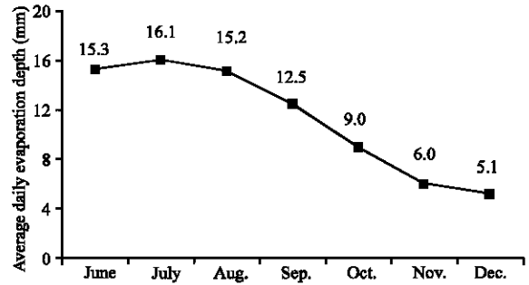
Fig. 1: Measured average daily pan evaporation depth (mm) from June-December
