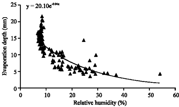
Fig. 4: A simple regression model for relative humidity and daily pan evaporation depth (mm)
