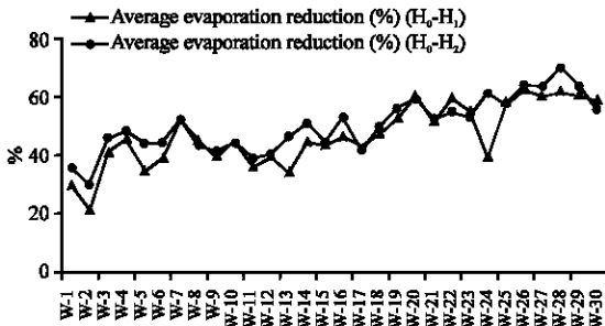
Fig. 6: Average weekly evaporation reduction (%) from evaporation pans ( H_0-H_1 ) and ( H_0-H_2 )
