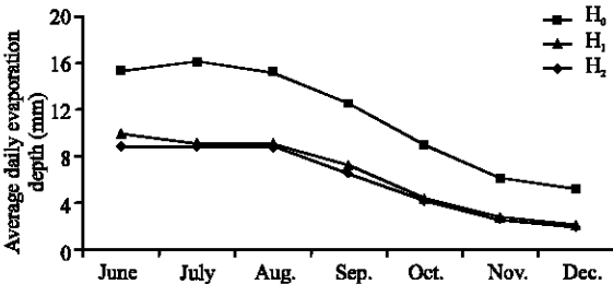
Fig. 5: Average daily evaporation depth (mm) measured for three evaporation pans ( H_0 , H_1 and H_2 )
