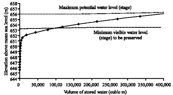
Fig. 7: Stage-volume curve for Al-Alb Dam, Riyadh, Saudi Arabia
