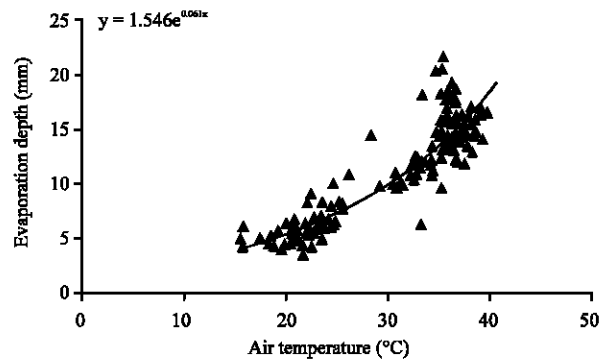
Fig. 2: A simple regression model for daily air temperature and daily evaporation depth (mm)
