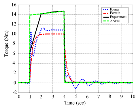
Fig. 5: Response of ANFIS, Riener and Ferrarin muscle models
