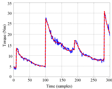
Fig. 3: Output from the testing data set, testing: output (-) and ANFIS output (-)
