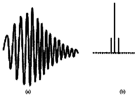
Fig. 2: Diagram of the intensity distribution of real ultrasound source
