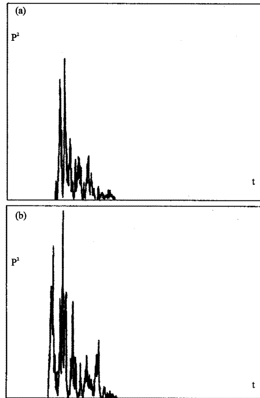
Fig. 5: Interference of ultrasound waves in the probe: a) P = 2.5 cm, a = 6 cm, \sigma = 18 cm 2 and b) P = 2 cm, a = 6 cm, \sigma = 16 cm 2
