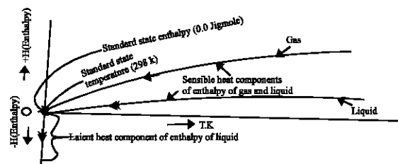
Fig. 1: Aschematic idealization of the calculation of the enthalpies of gases and liquids relative to the standard state (the gas at 298 K and 1 atm)
