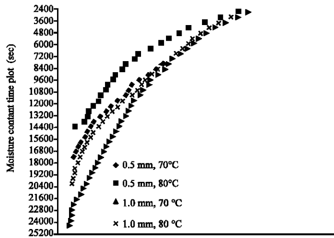
Fig. 1: The equilibrium moisture content versus time
