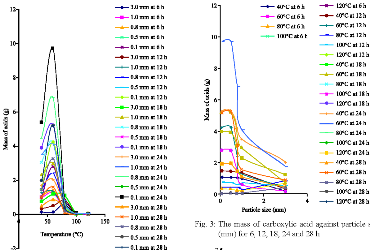
Fig. 2: The mass of carboxylic acid against temperature (°C) for 6, 12, 18, 24 and 28 h
