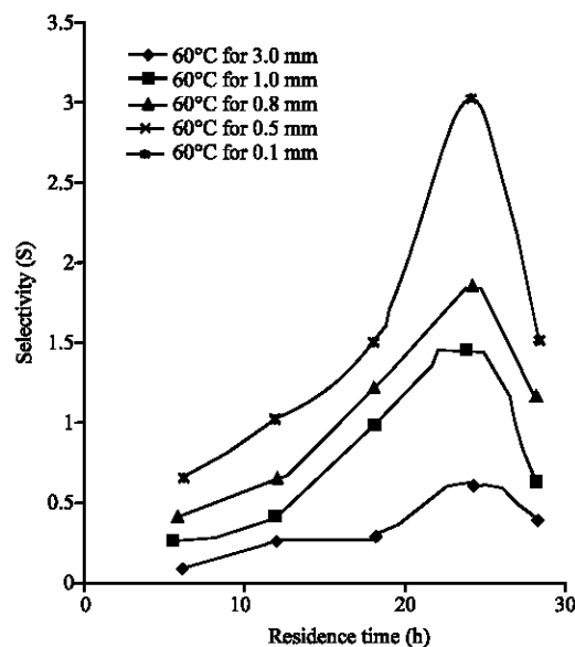
Fig. 4: The Selectivity (S) against residence time at 60°C
