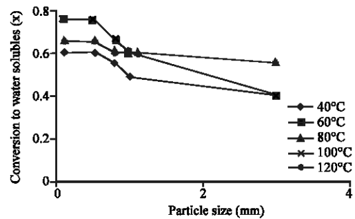
Fig. 9: The conversion to water soluble (X) against particle size for 24 h
