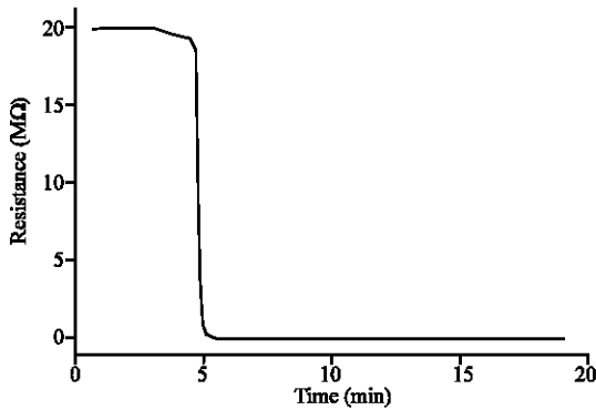
Fig. 2: Variation of the internal resistance of the Lambda sensor during heating period
