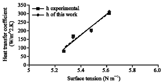
Fig. 5: Surface tension vs. heat transfer coefficient at test section inlet pressure = 3200 kPa and different volume flow rate
