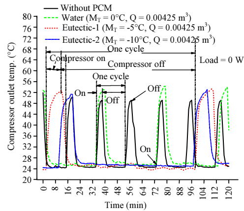
Fig. 5: The effect of PCM on compressor on/off cycling (L = 0 W, Q = 0.00425 m 3 )
