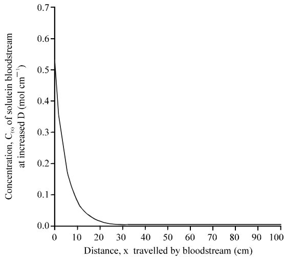
Fig. 6: Graph of concentration of solute C_{(x)} at increased D against distance, x
