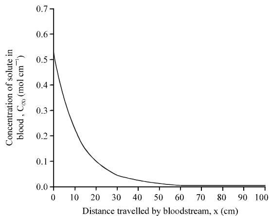
Fig. 4: Graph of concentration of solute C_{(x)} against distance, x without D, V, R
