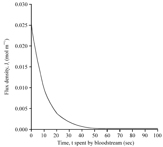
Fig. 13: Graph of flux density, J , against time, t
