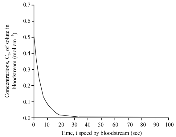
Fig. 3: Graph of concentration of solute C_{(t)} against time, t
