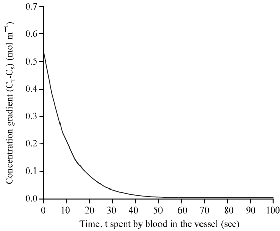
Fig. 11: Graph of Concentration gradient, ( C_t-C_s ) against time, t
