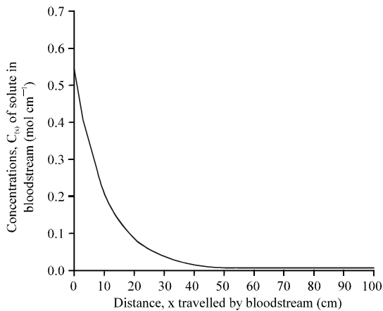
Fig. 2: Graph of concentration of solute C_{(x)} against distance, x
