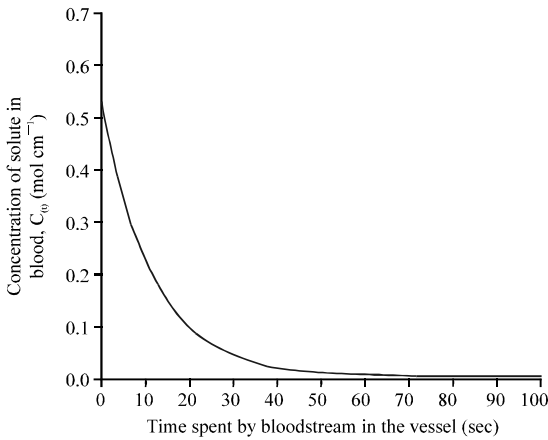
Fig. 5: Graph of concentration of solute in blood against time, t without D , V , R
