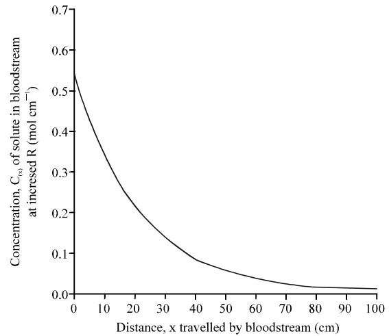
Fig. 7: Graph of concentration of solute C_{(x)} at increased R against distance, x
