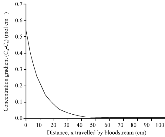
Fig. 10: Graph of concentration gradient ( C_x-C_s ) against distance, x
