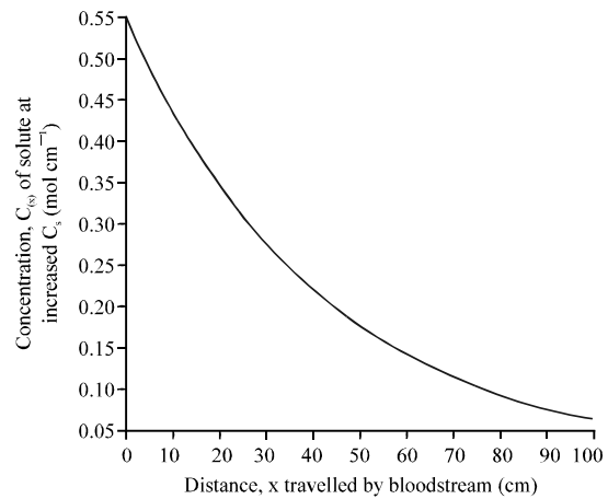
Fig. 8: Graph of concentration of solute C_{(x)} at increased C_s against distance, x
