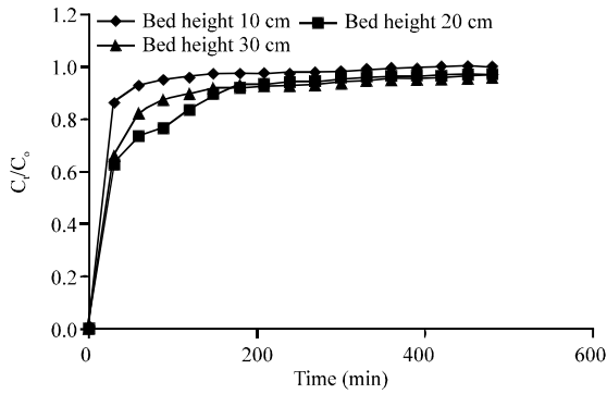
Fig. 4: Breakthrough curves for the adsorption of metanil yellow on H_3PO_4 -activated carbon
