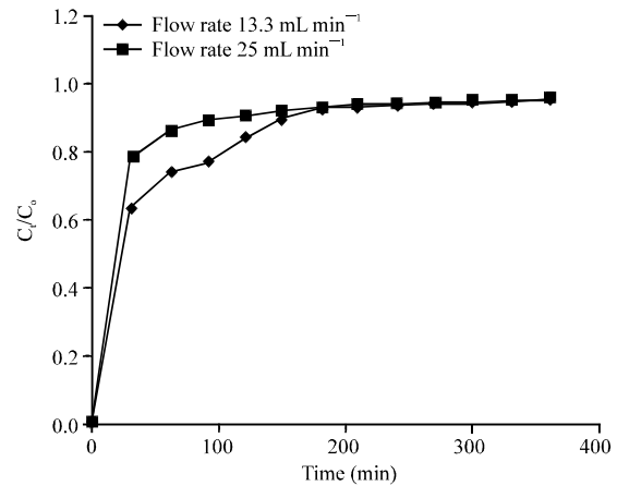
Fig. 8: Breakthrough curves for the adsorption of metanil yellow on H_3PO_4 -activated carbon at initial influent concentration C_0 10 \text{ mg L}^{-1}
