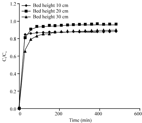
Fig. 6: Breakthrough curves for the adsorption of metanil yellow on H_3PO_4 -activated carbon at influent concentration C_0 50 \text{ mg L}^{-1}
