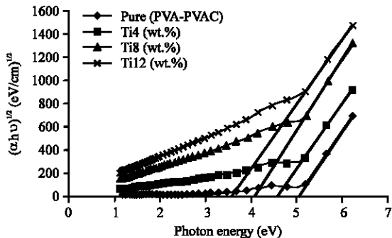
Fig. 3: The relationship between (\alpha h\nu)^{1/2} (eV/cm) 1/2 and photon energy of (PVA-PVAC-Ti) nanocomposites
