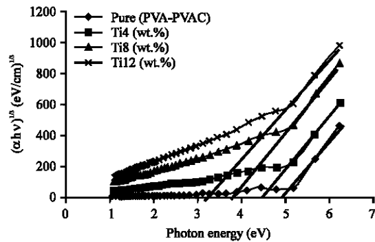
Fig. 4: The relationship between (\alpha h\nu)^{1/3} (eV/cm) 1/3 and photon energy of (PVA-PVAC-Ti) nanocomposites
