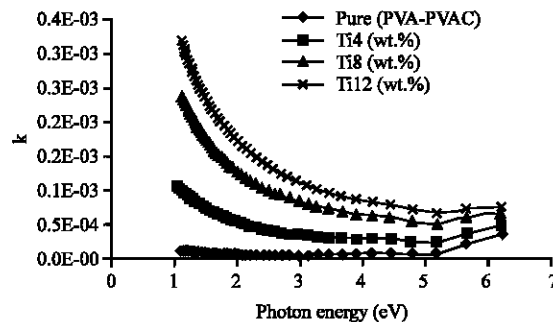
Fig. 5: The relationship between extinction coefficient (PVA-PVAC-Ti) nanocomposites with photon energy
