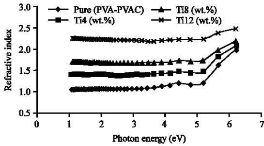
Fig. 6: The relationship between refractive index (PVA-PVAC-Ti) nanocomposite with photon energy
