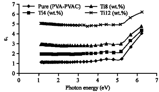
Fig. 7: The relationship between realparts of dielectric constant (PVA-PVAC-Ti) nanocomposite with photon energy
