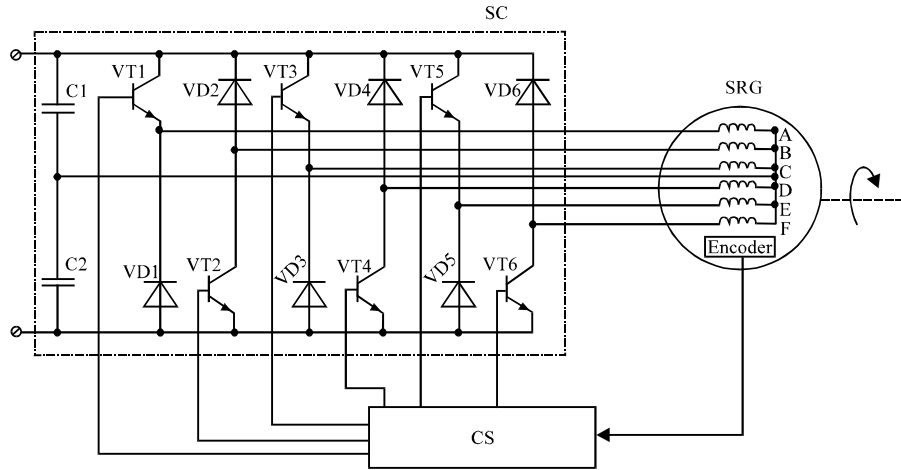
Fig. 1: Scheme of six-phase SRG and supply converter (SC: Static Converter; CS: Control System; Encoder-rotor position sensor)
