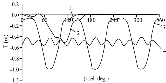
Fig. 3: Dependence of SRG electromagnetic torques (1-torque of single phase of SRG 18/12, 2-torque of single phase of SRG 18/15, 3-total torque of SRG 18/12, 4-total torque of SRG 18/15)
