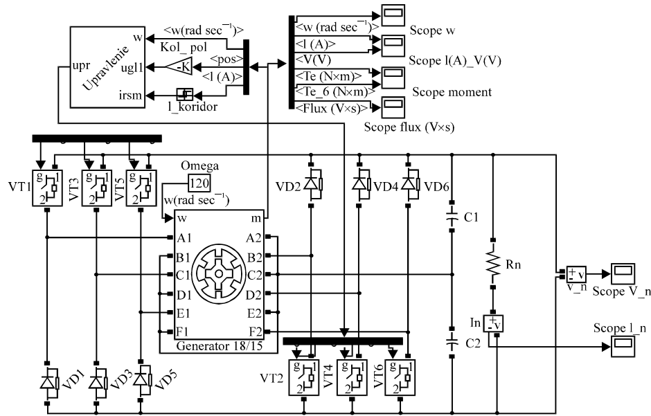
Fig. 2: Computer model of six-phase SRG 18/15 configuration
