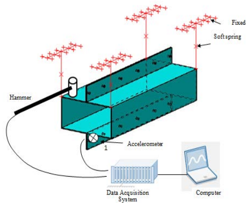
Fig. 4: Experimental setup
