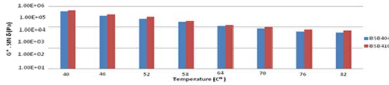
Fig. 19: G* sind test for samples containing 4% SBS and 4% sulphur (G* sinδ (Pa))
