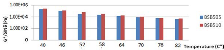
Fig. 22: G*/sind test for samples containing 4% SBS and 5% sulphur (G* sinδ (Pa))
