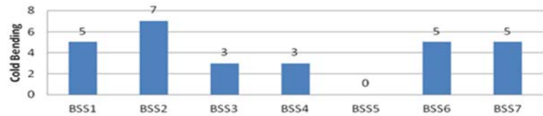
Fig. 8: Cold Bending result for Bitumen-SBS-sulphur mixtures
