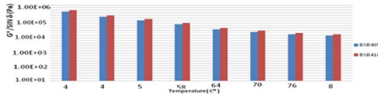
Fig. 18: G* / sin delta test for samples containing 4% SBS and 4% sulphur
