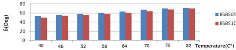
Fig. 21: d test for samples containing 4% SBS and 5% sulphur (δ (deg))
