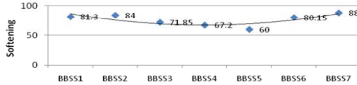
Fig. 24: Softening point result for Bitumen-SBS-sulphur and pure bentonite mixtures
