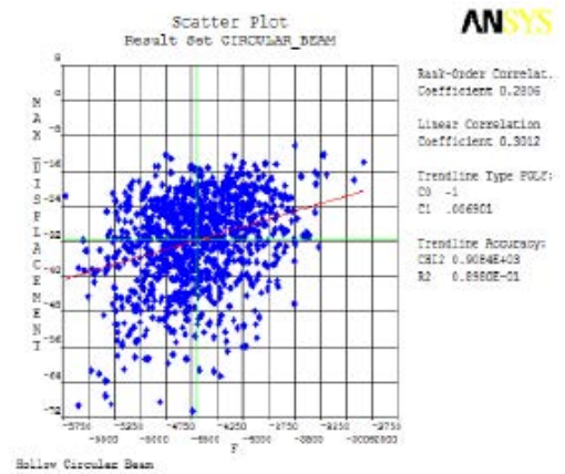
Fig. 17: Scatter plot of maximum deflection vs. load of hollow circular composite beam
